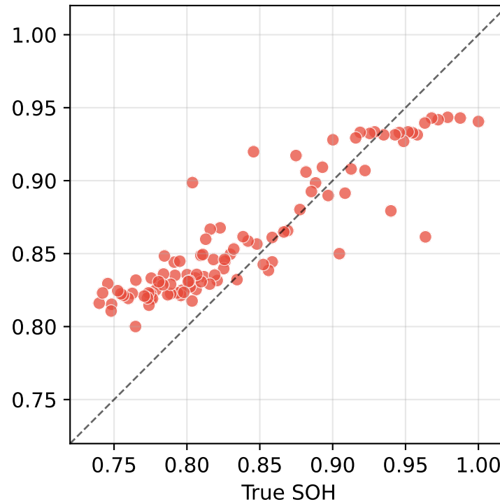
MSc Model: Predicted vs True SOH (Validation Set)
