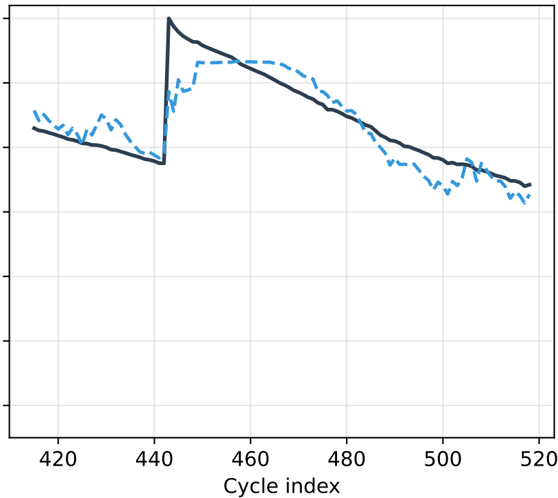
Validation SOH Trajectories (Paper Reproduction)
