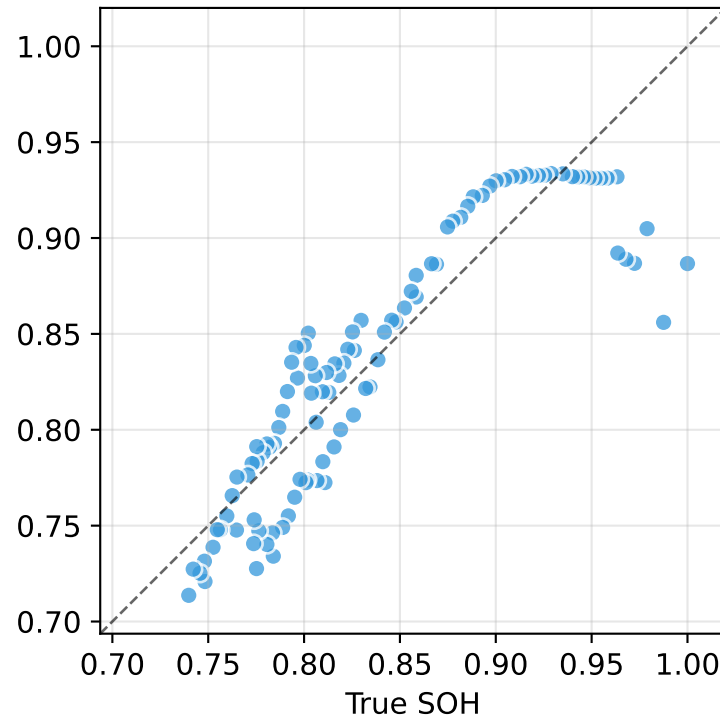
Predicted vs True SOH (Validation Set) Oxford
