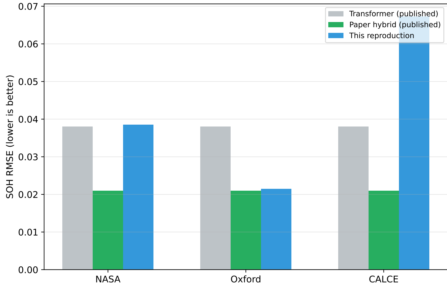
SOH RMSE vs Published Baselines
