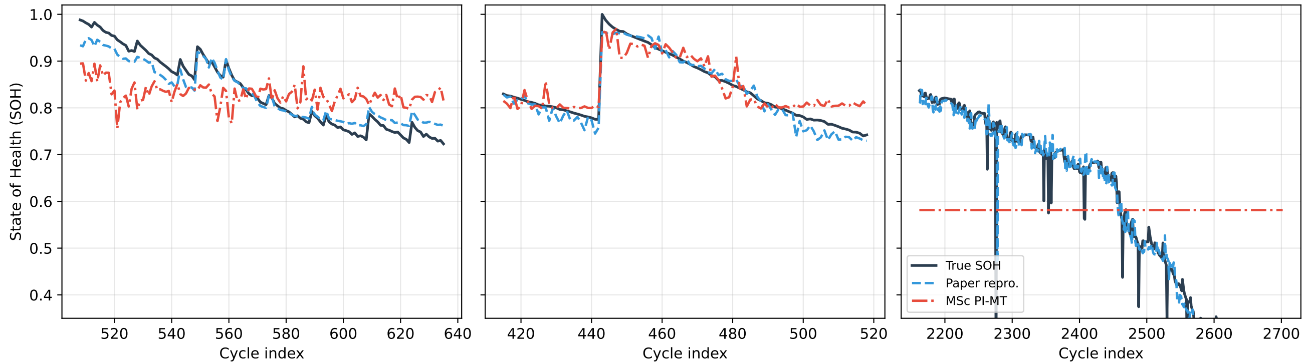
Validation SOH Trajectories: Paper Reproduction vs MSc Extension
