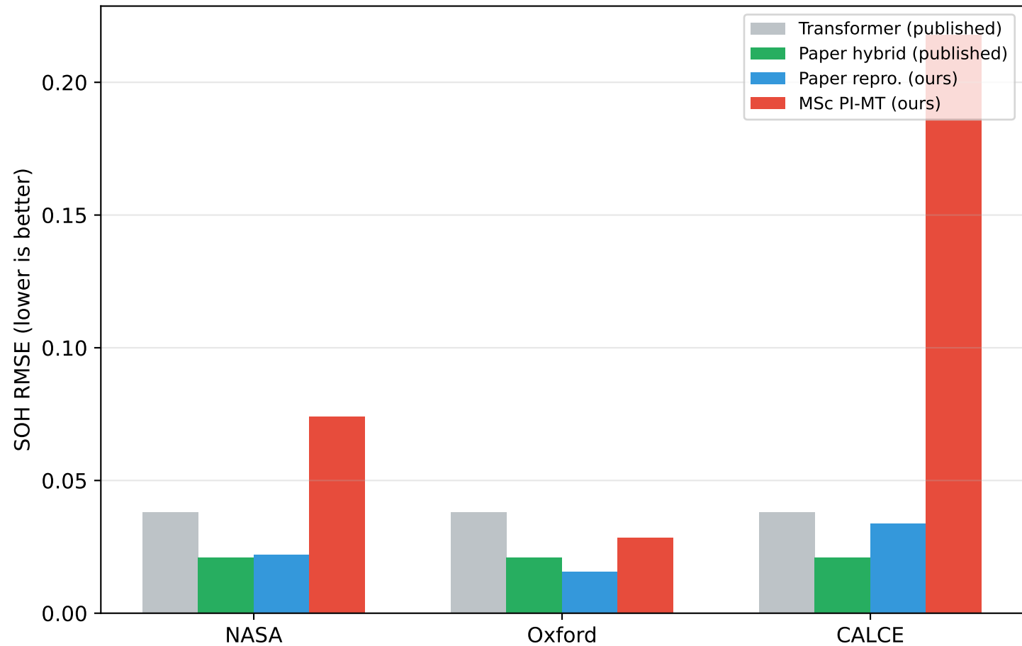
SOH RMSE Comparison Across Datasets
