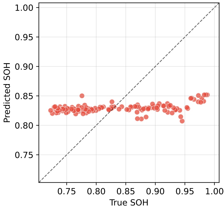
MSc Model: Predicted vs True SOH (Validation Set) NASA
