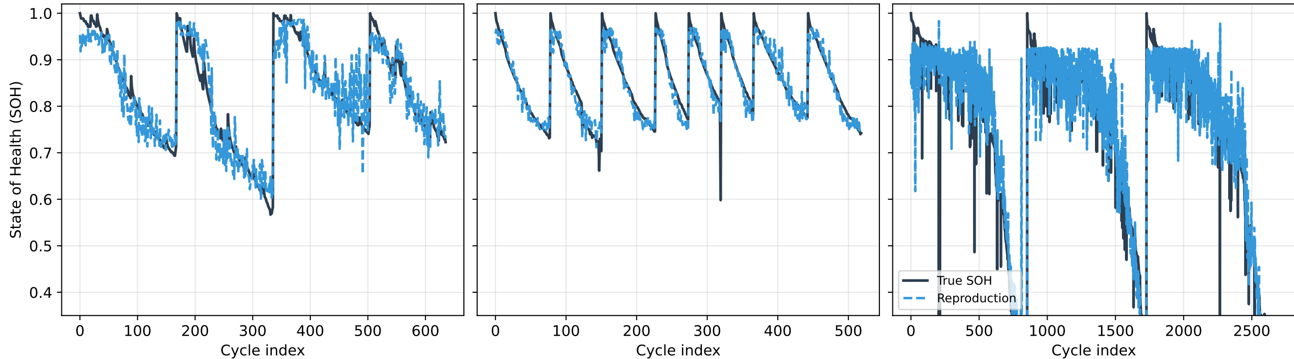
SOH Trajectories (stratified_5fold_cv_pooled_oof)
