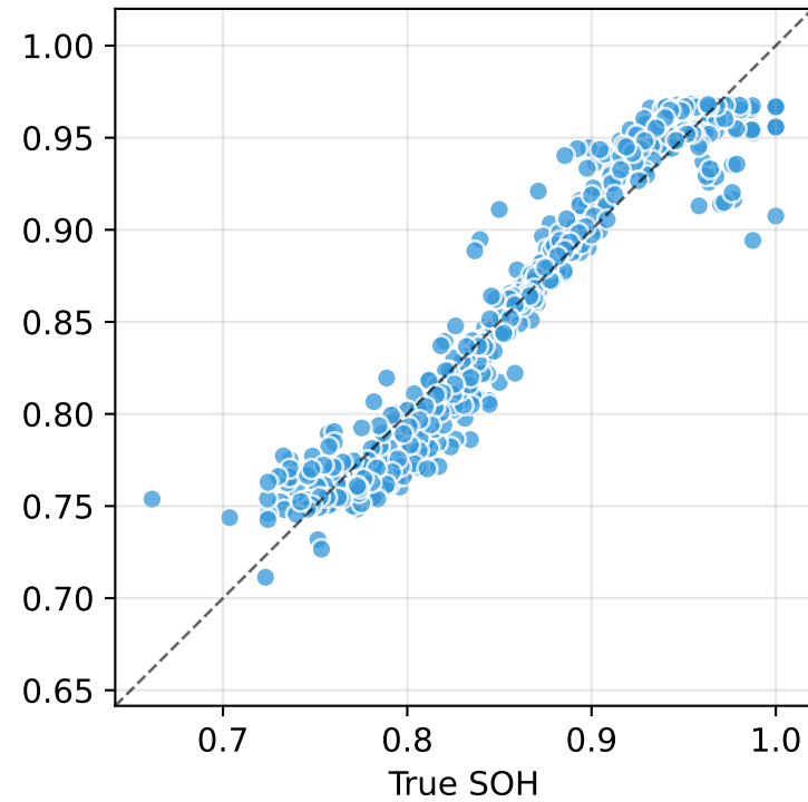
Predicted vs True SOH (stratified_5fold_cv_pooled_oof)
