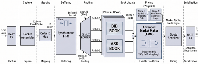
Fig. 1. Top-level System Architecture of HFT Datapath, illustrating the flow from the physical layer interface through packet parsing, order book management, and trading logic.
