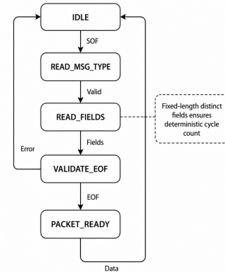
Fig. 3. State transition diagram of the packet parser, highlighting the fixed-length field extraction sequence.
