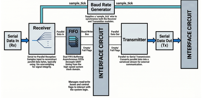
Fig. 2. Physical layer interface utilizing custom UART core with input FIFOs to ensure cycle-accurate data ingestion.
