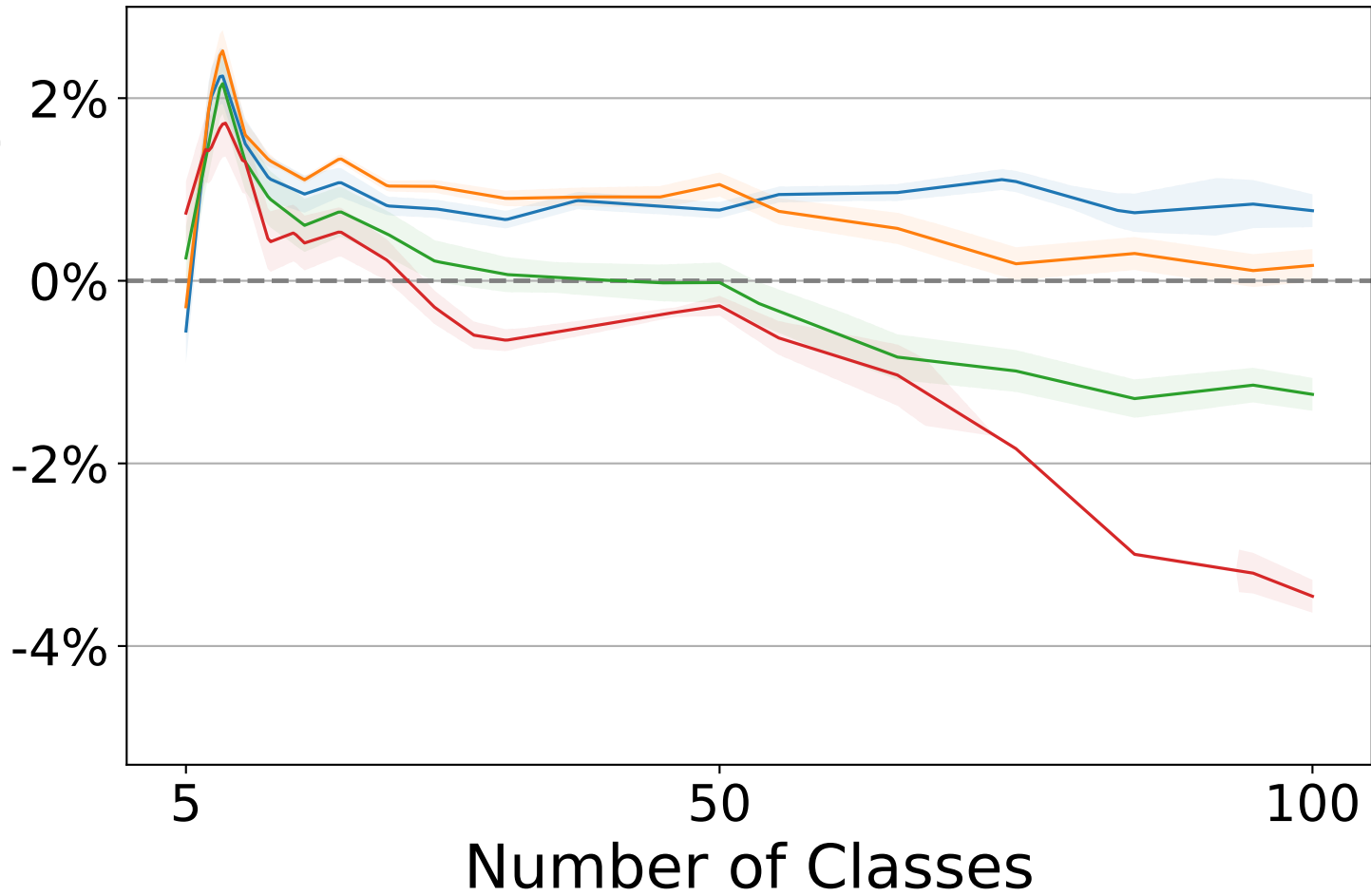
Relative Accuracy
