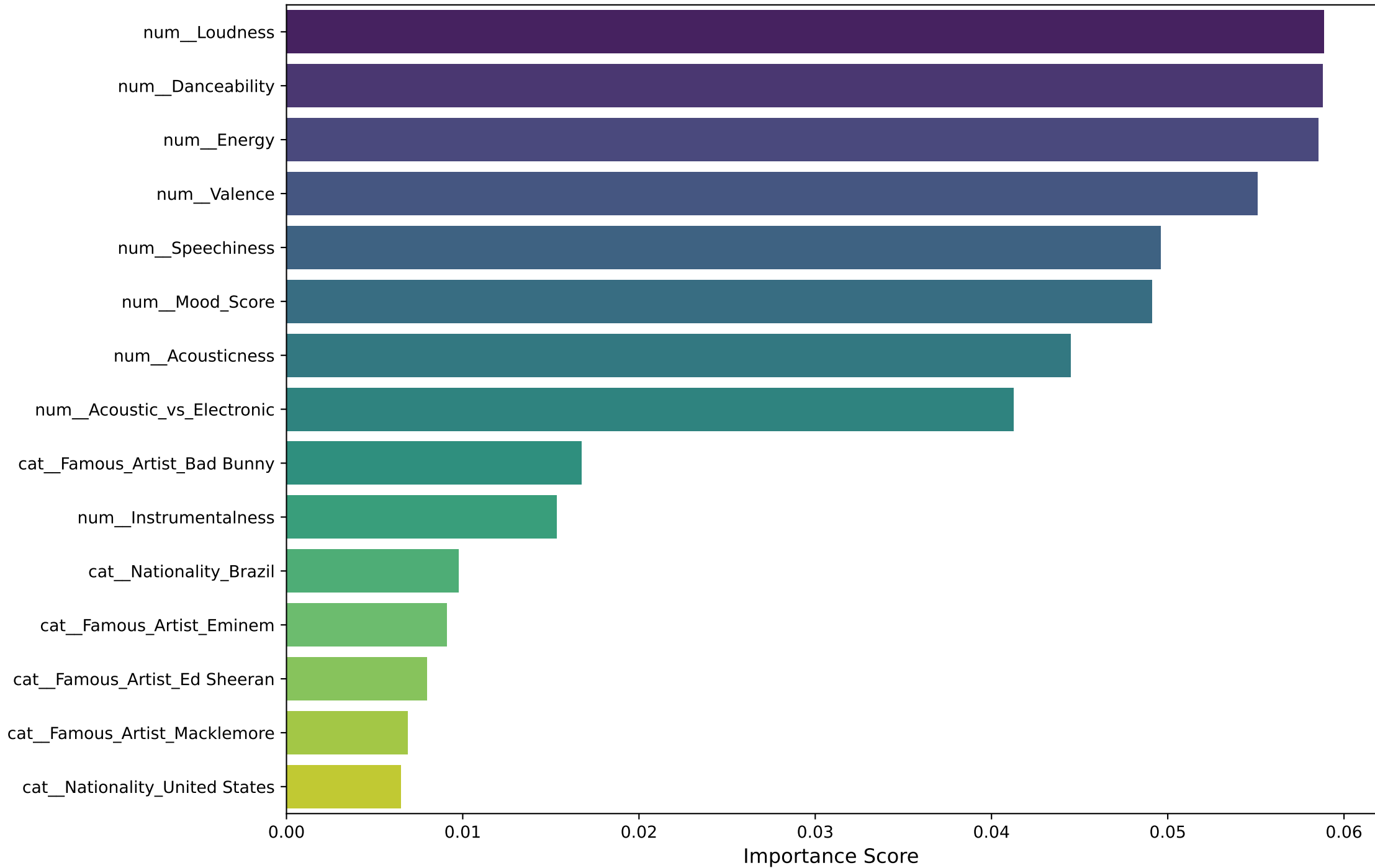
Top 15 Feature Importances (from Extra Trees (Tuned))
