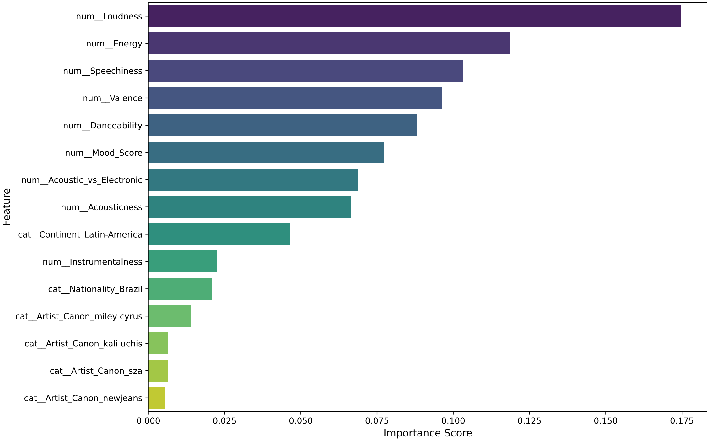
Top 15 Feature Importances (from Random Forest)
