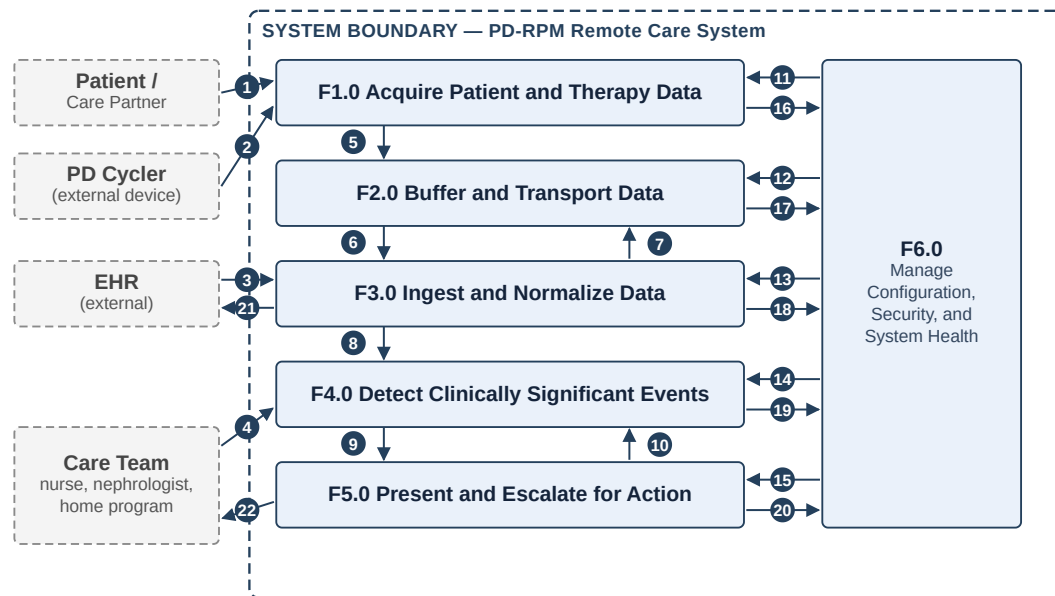
Figure 1. Level 1 functional diagram. Boxes inside the dashed boundary are functions the system performs; gray dashed boxes are external elements it interfaces with but does not perform. Numbered circles key to Table 1.
