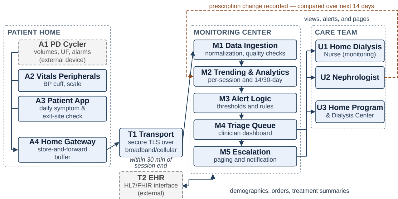
Figure 1. PD-RPM system concept. Solid arrows carry data; the brown dashed arrow is the clinician feedback path; gray dashed boxes lie outside the system boundary.
