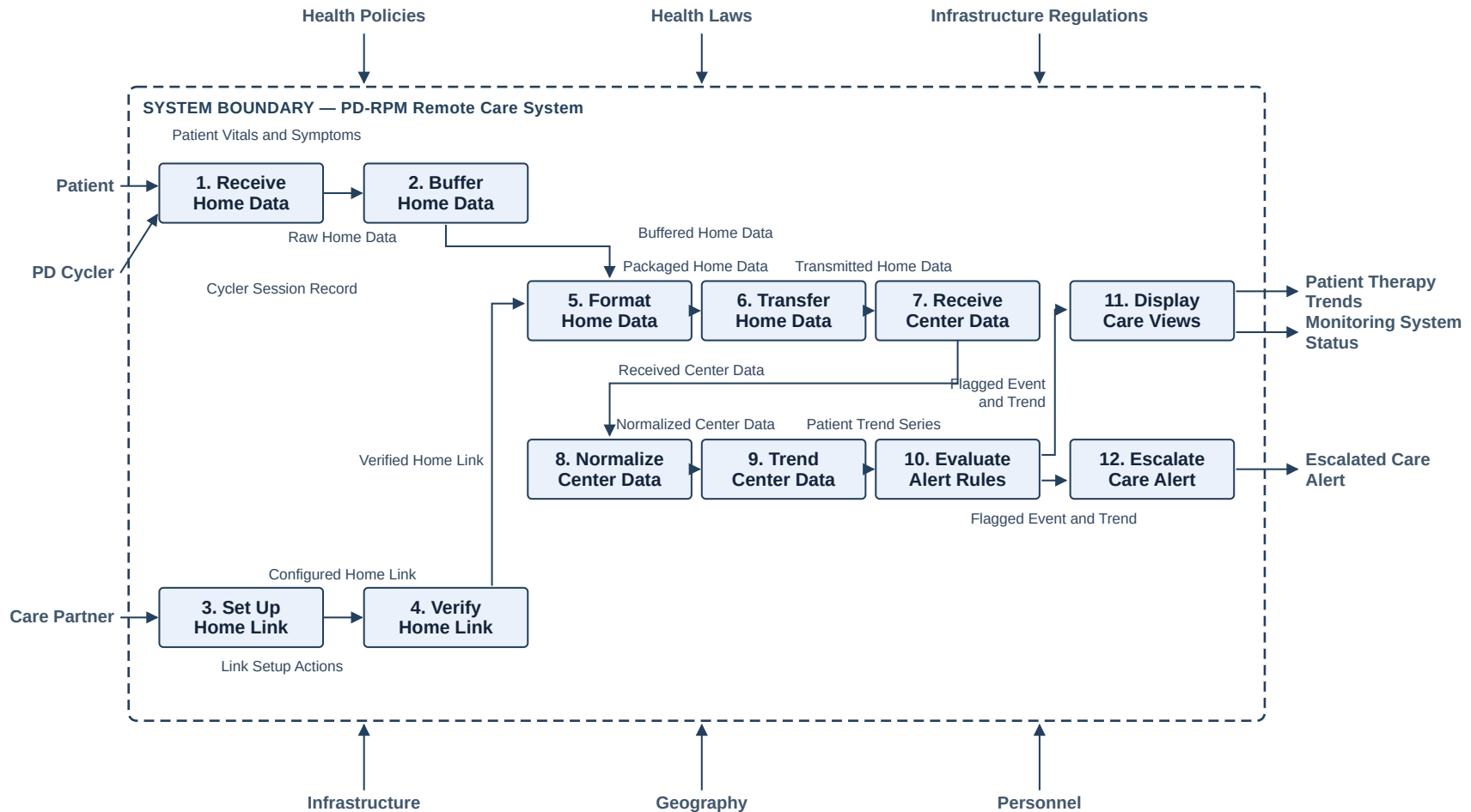
Figure 1. Level 1 functional diagram, drawn as a functional overlay on the PD-RPM context diagram. Twelve verb-noun functions; every flow labeled with the noun that passes.
