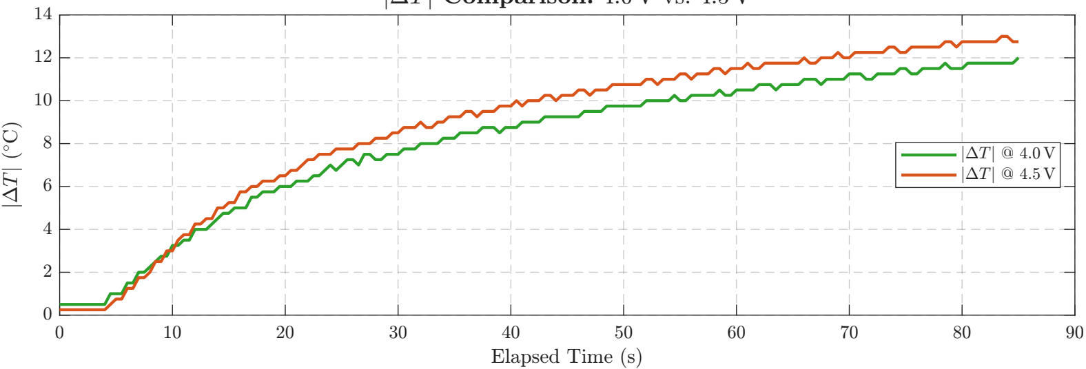
|\Delta T| Comparison: 4.0 V vs. 4.5 V
