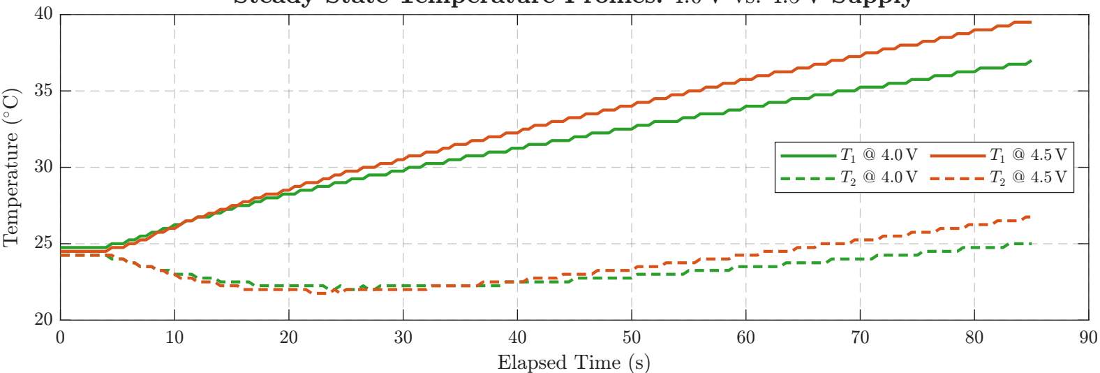
Steady-State Temperature Profiles: 4.0 V vs. 4.5 V Supply
