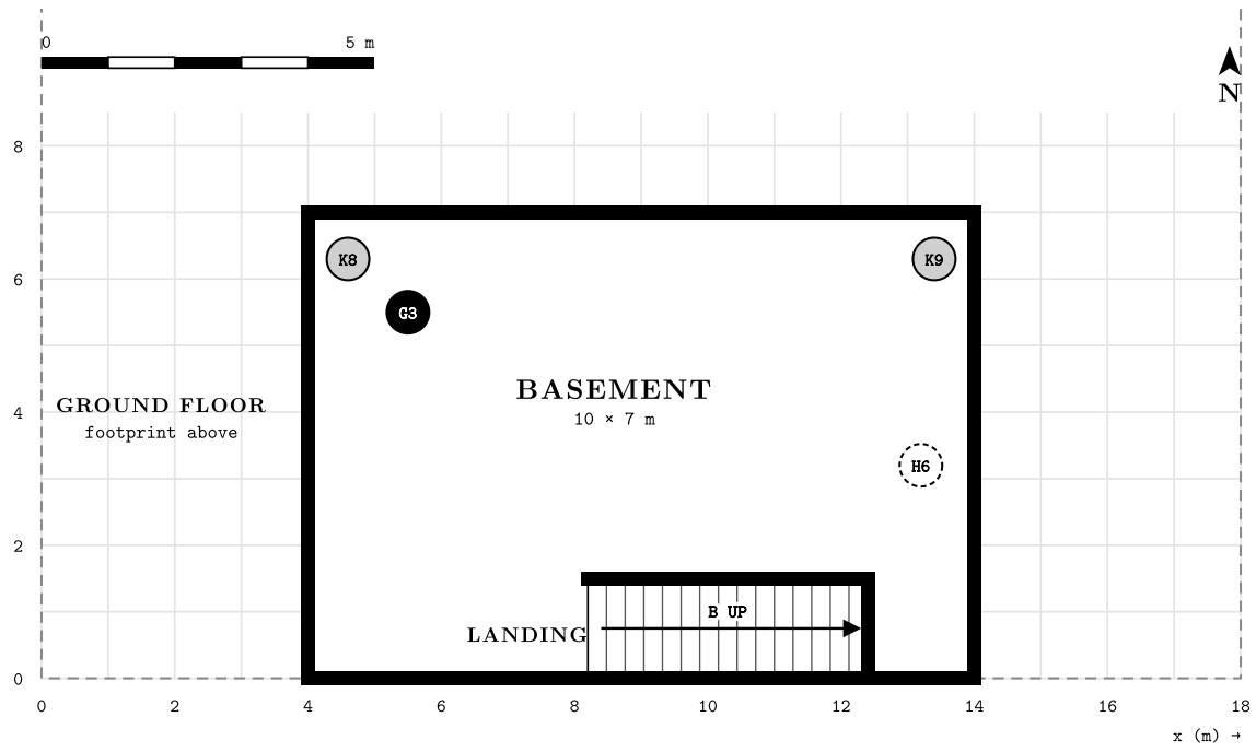
Figure 3: Basement, y = -3 . One 10 \times 7 m room reached only by stairs B. The dashed outline is the ground floor above, for alignment.
