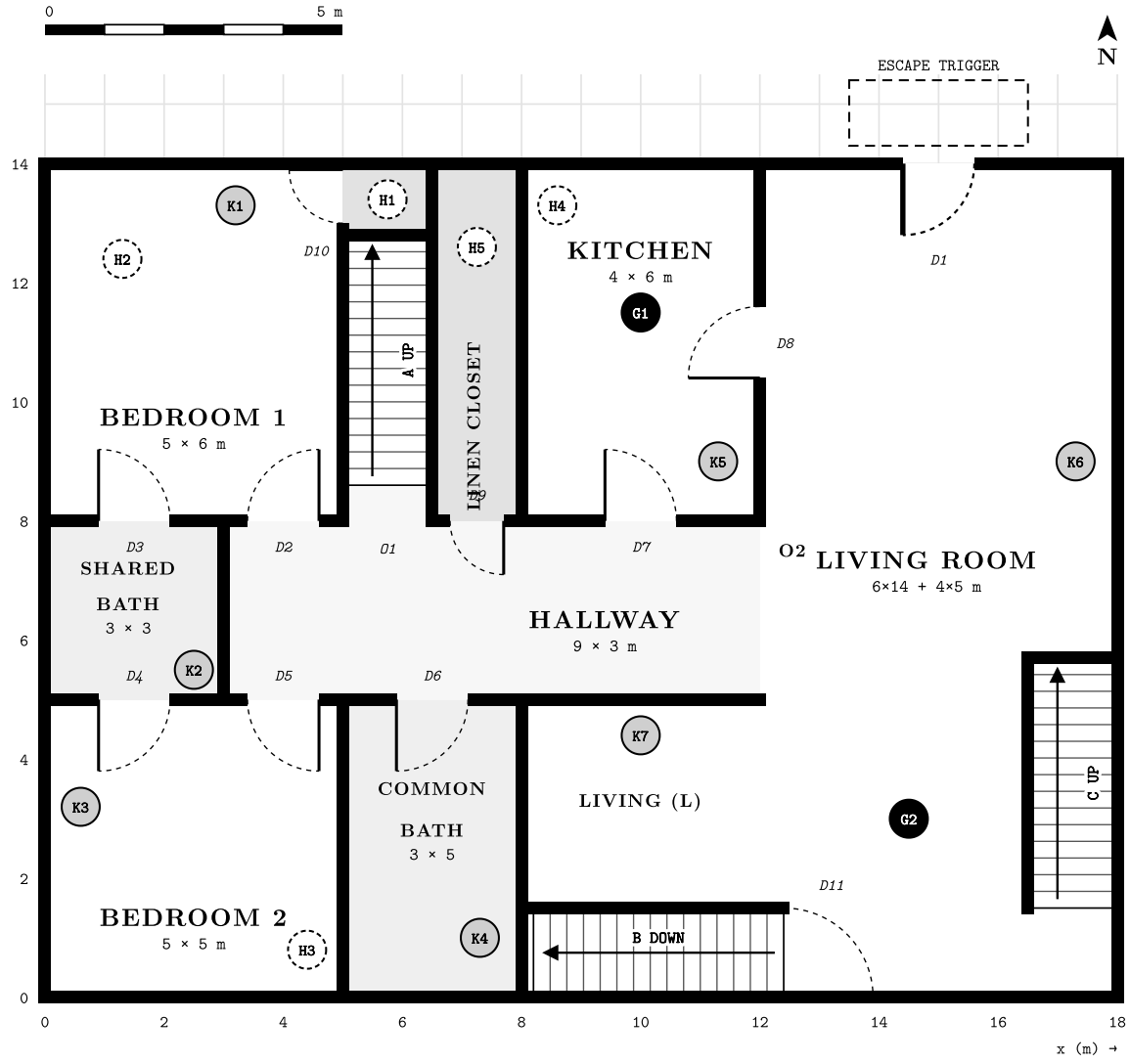
Figure 2: Ground floor, y = 0 . Footprint 18 \times 14 m. The front door D1 is the only exit; the escape trigger sits just outside it.
