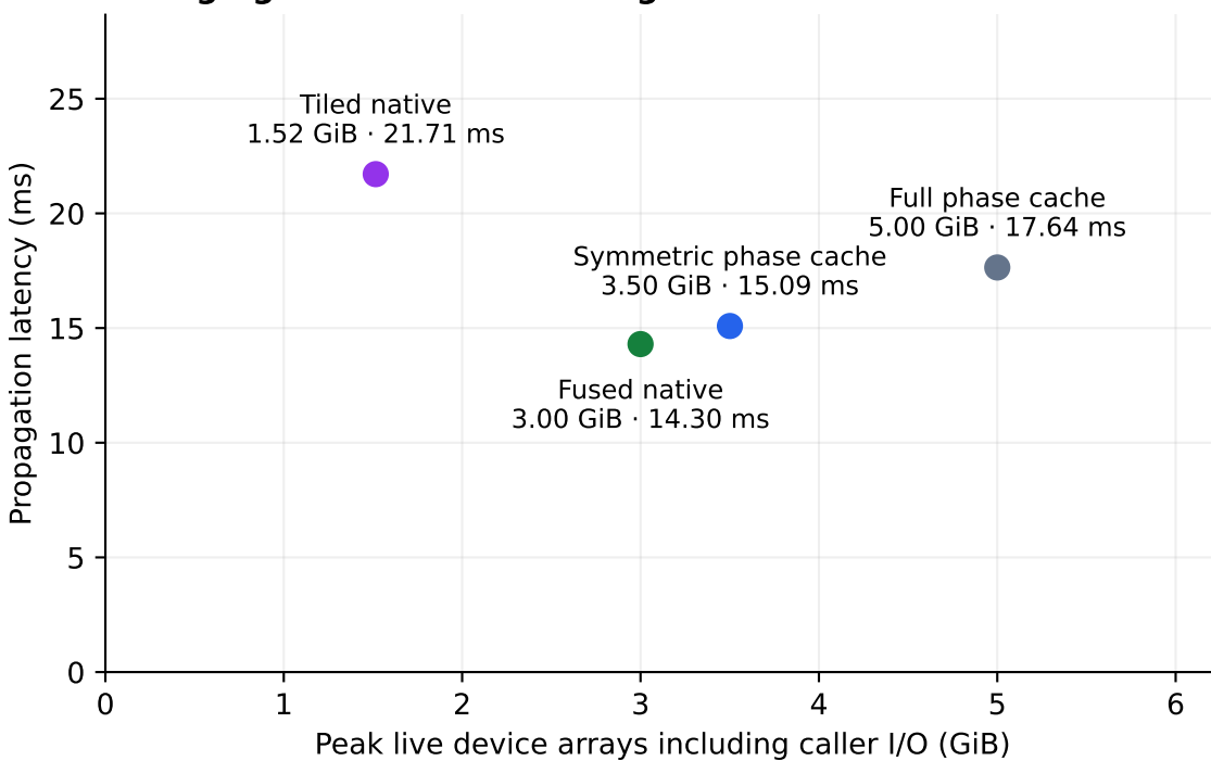
Changing distance + wavelength · 4096 × 16384
