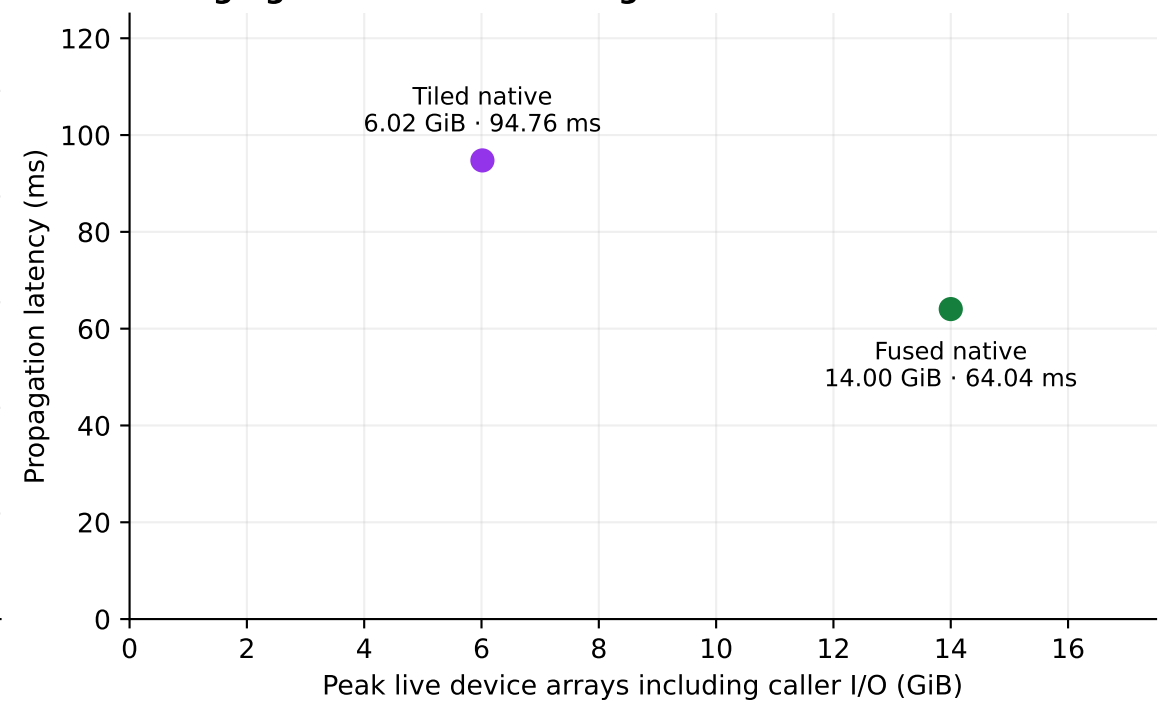
Changing distance + wavelength · 32768 × 8192
