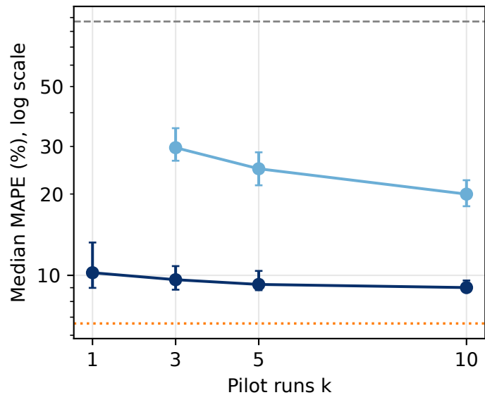
BUTTER-E \rightarrow EC-NAS
