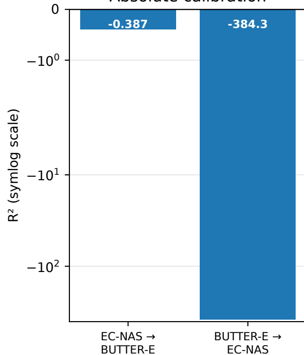
Absolute calibration
