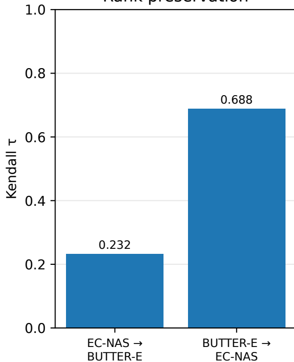
Rank preservation
