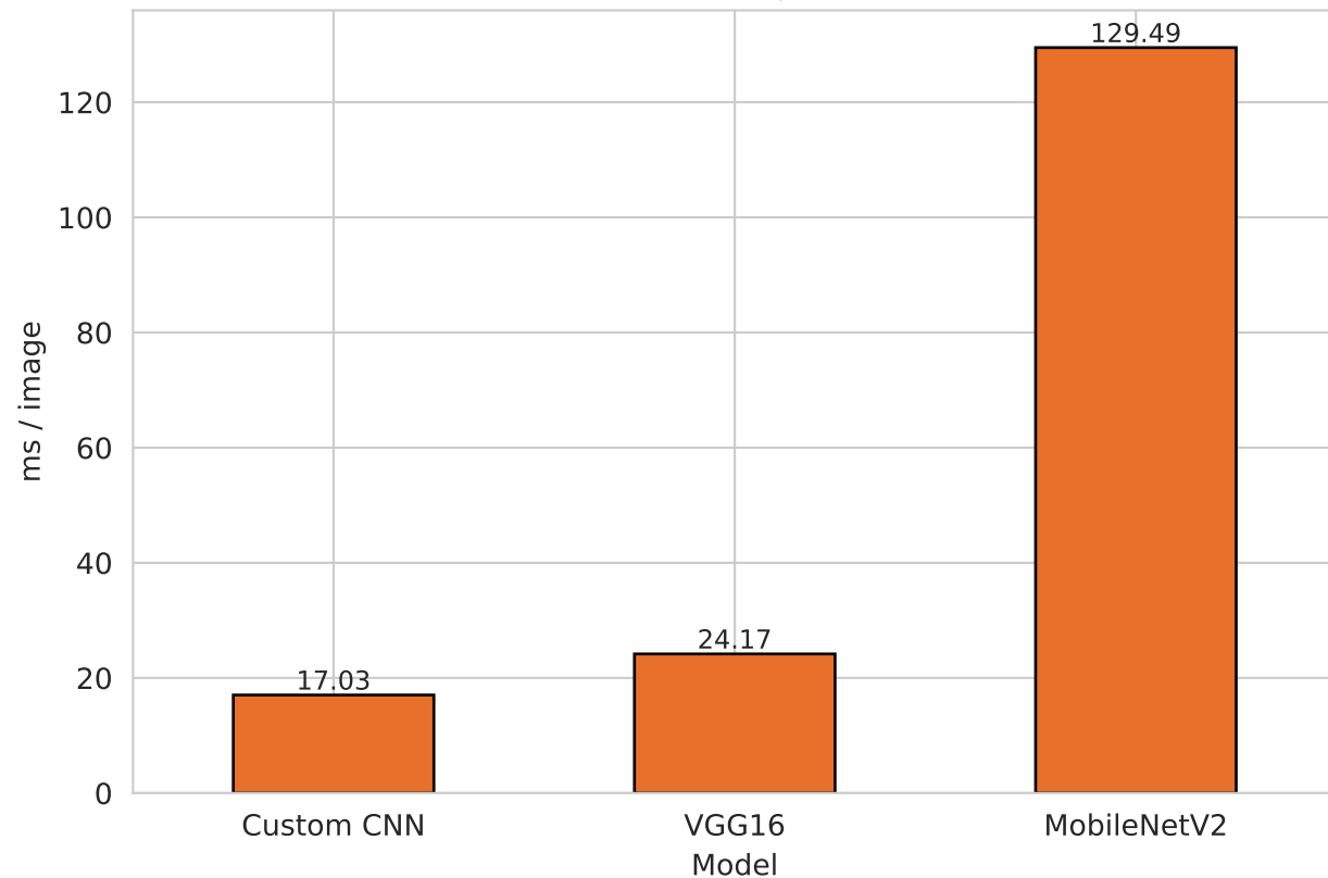
Inference Latency (batch=1)
