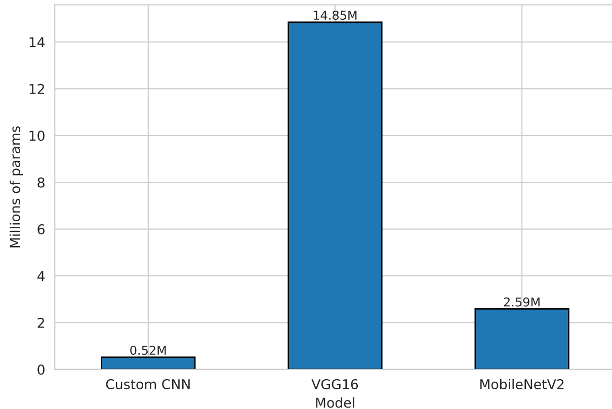
Model Size (Total Parameters)
