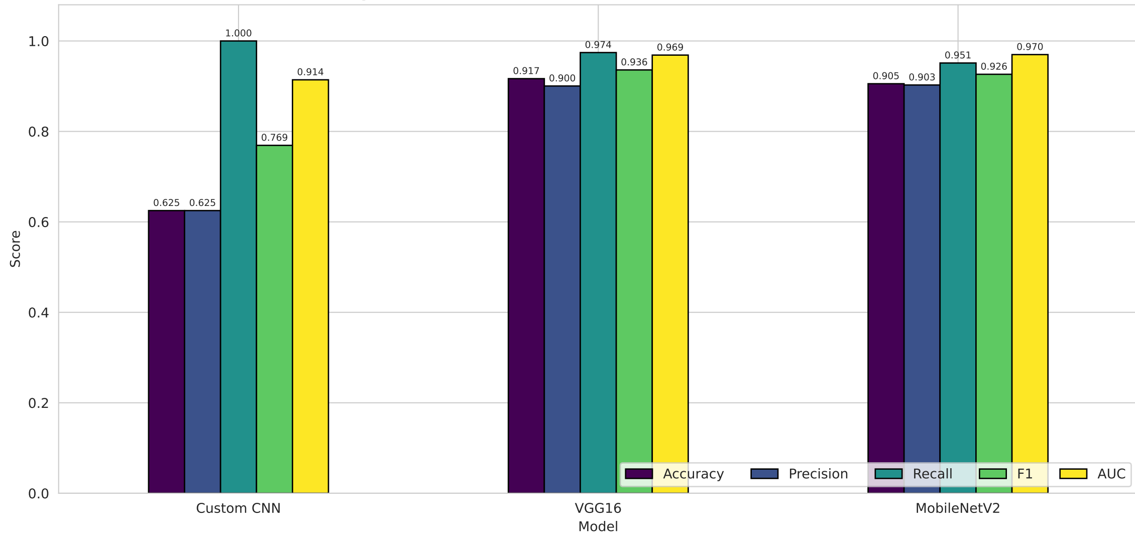
Model Comparison -- Test Metrics (Custom CNN vs VGG16 vs MobileNetV2)
