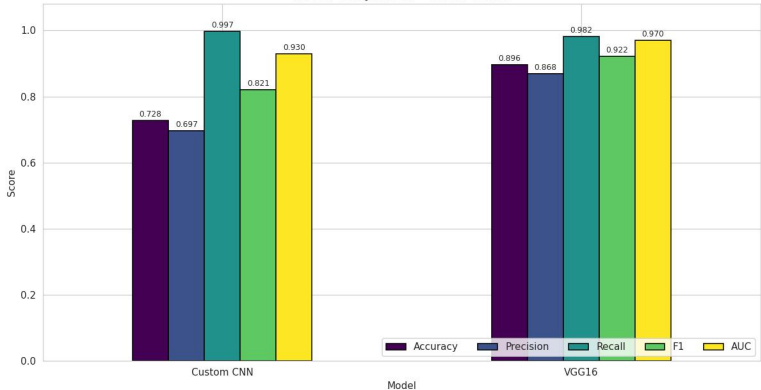
Model Comparison -- Test Metrics
