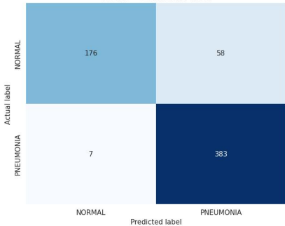
VGG16 -- Confusion Matrix
