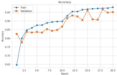
VGG16 Transfer Learning — Training Curves (Phase 1 + Phase 2)
