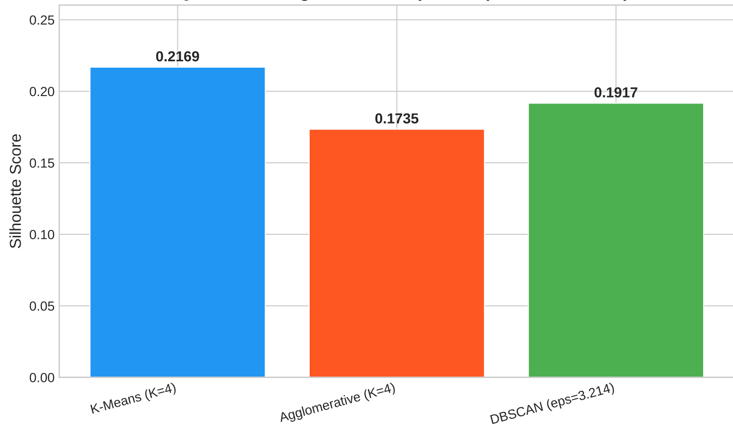
RQ3 — Clustering Method Comparison (Silhouette Score)
