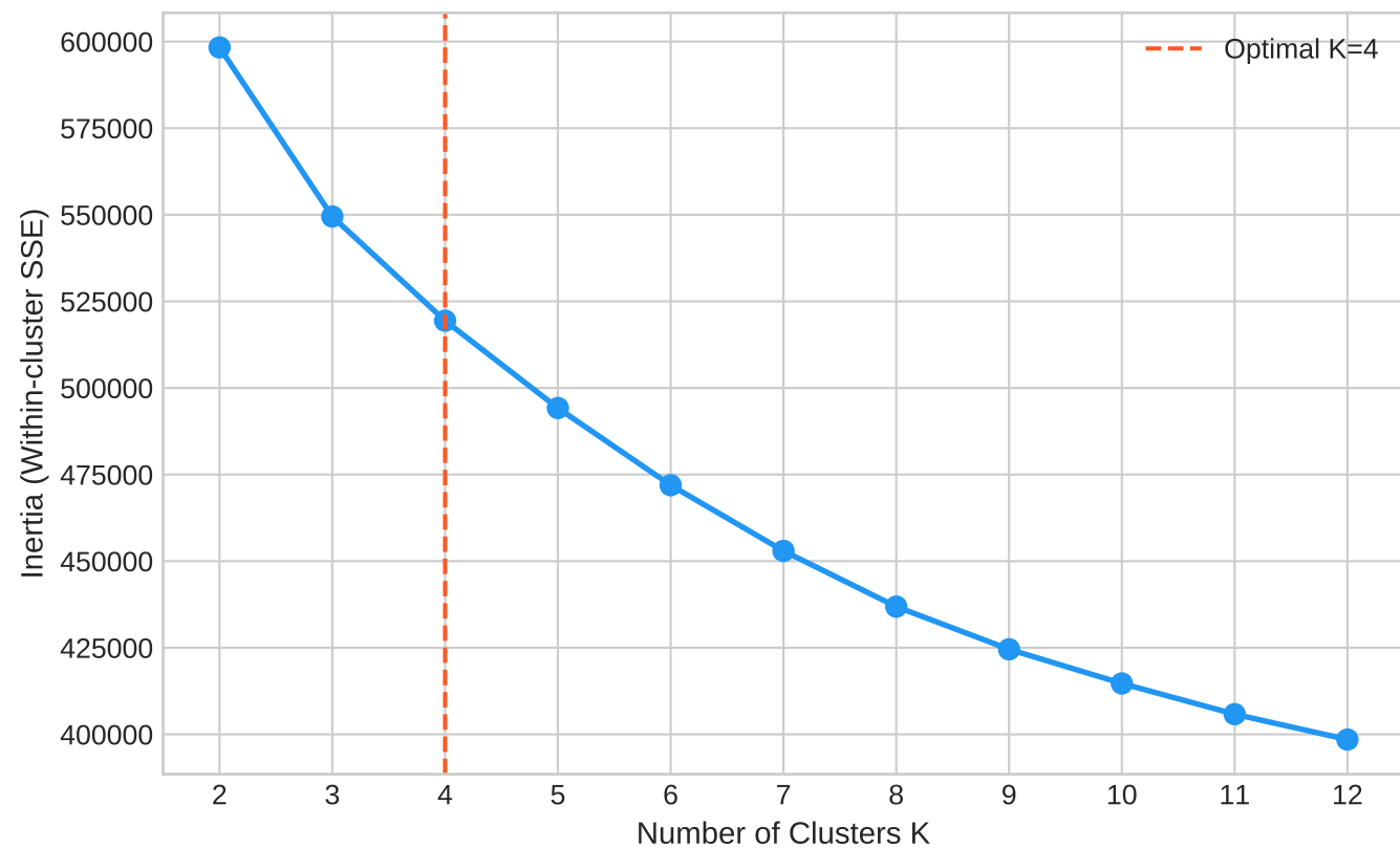
Elbow Method
