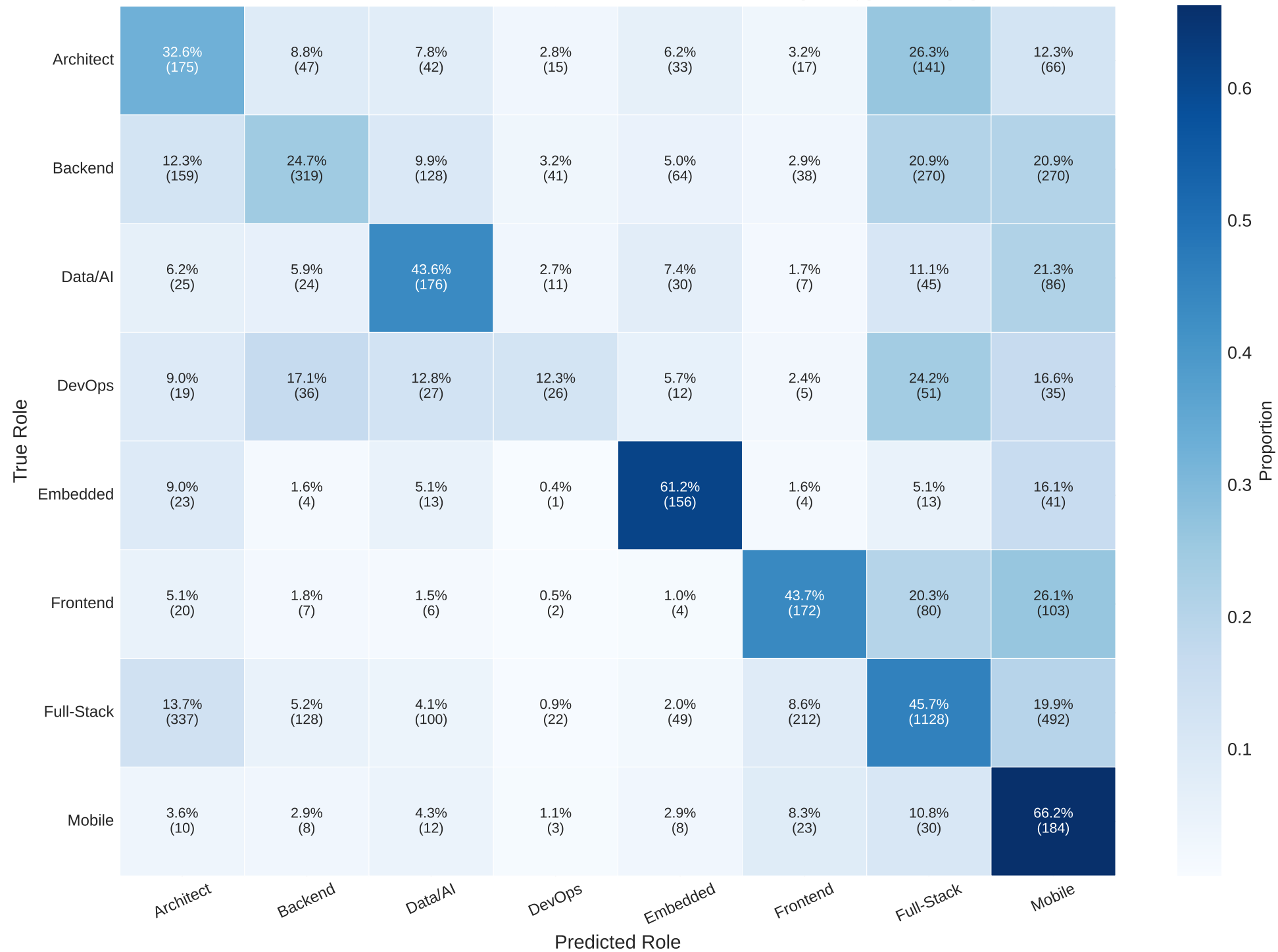
RQ7 — Normalized Confusion Matrix: Random Forest (DevType Groups)
