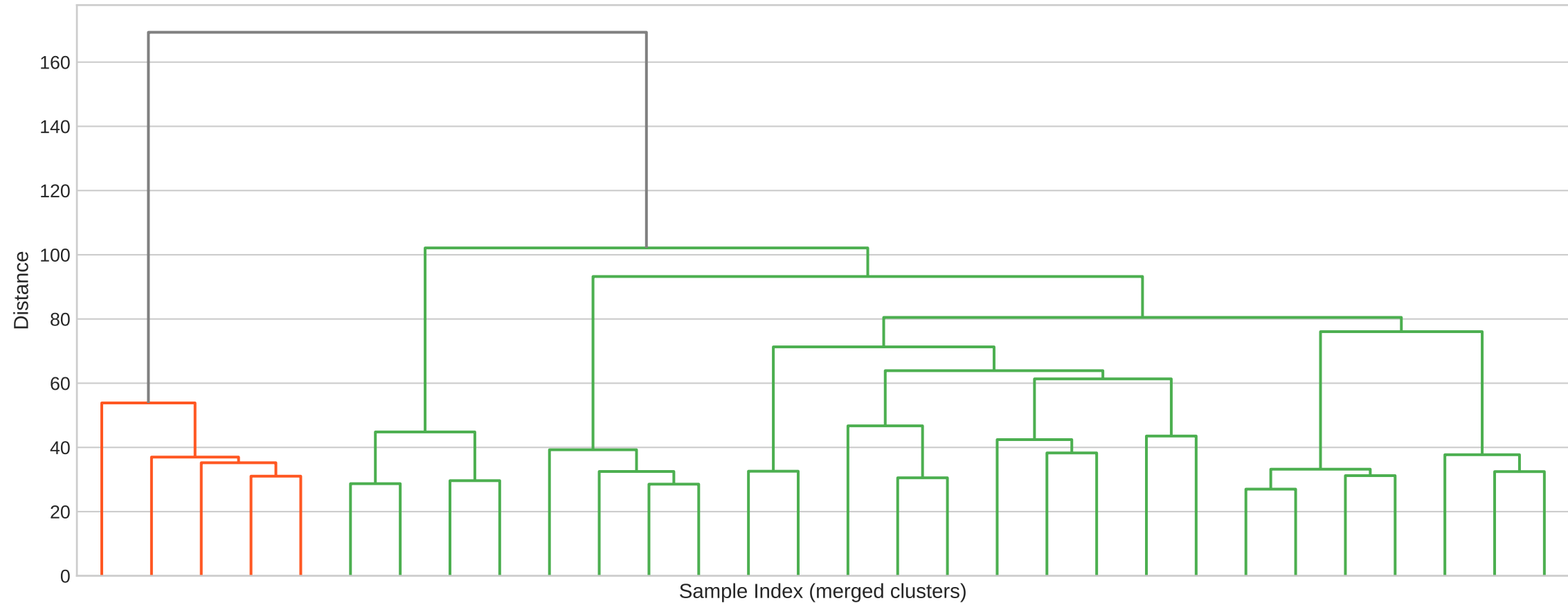
RQ3 — Ward Linkage Dendrogram (n=5,000 sample)
