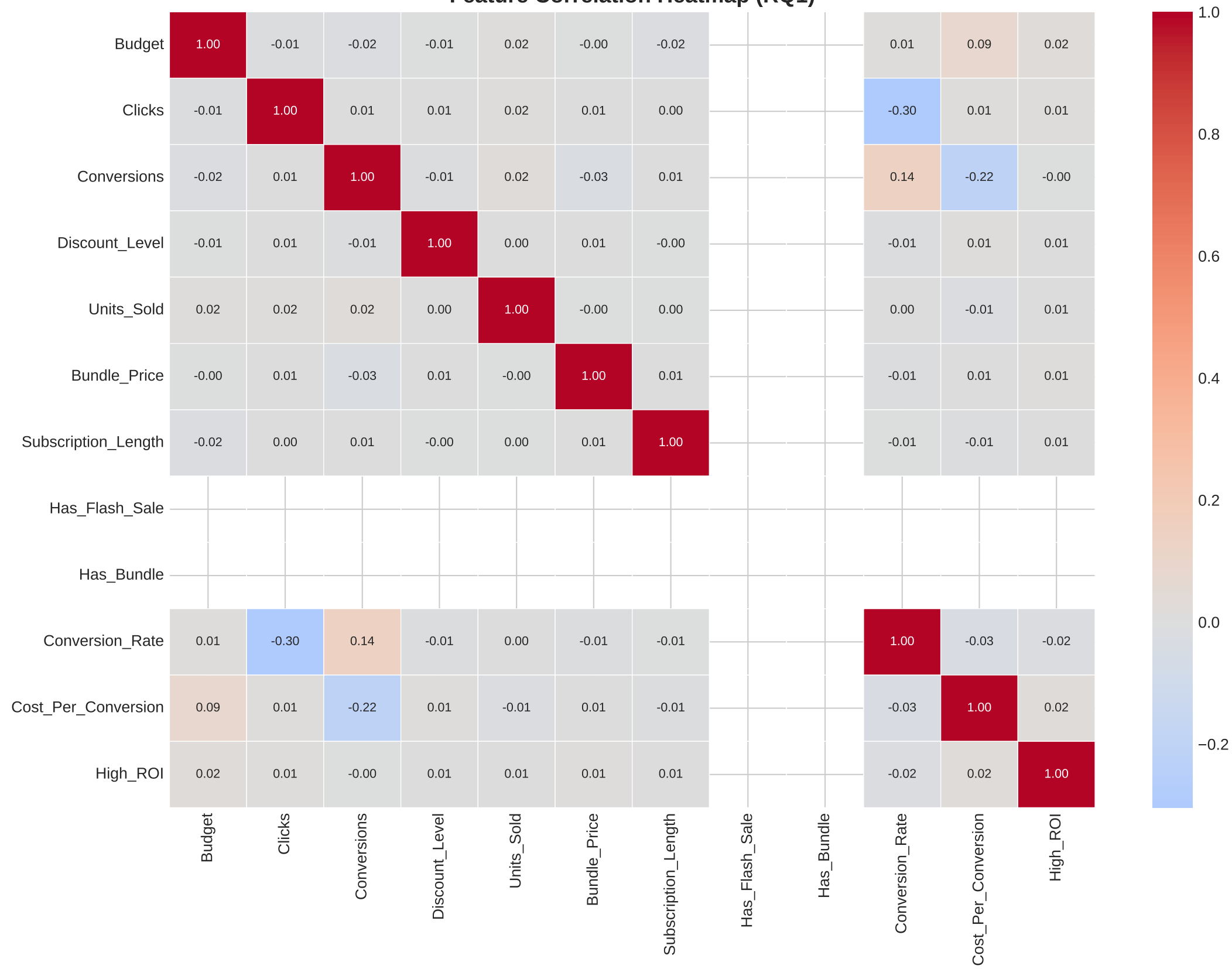
Feature Correlation Heatmap (RQ1)
