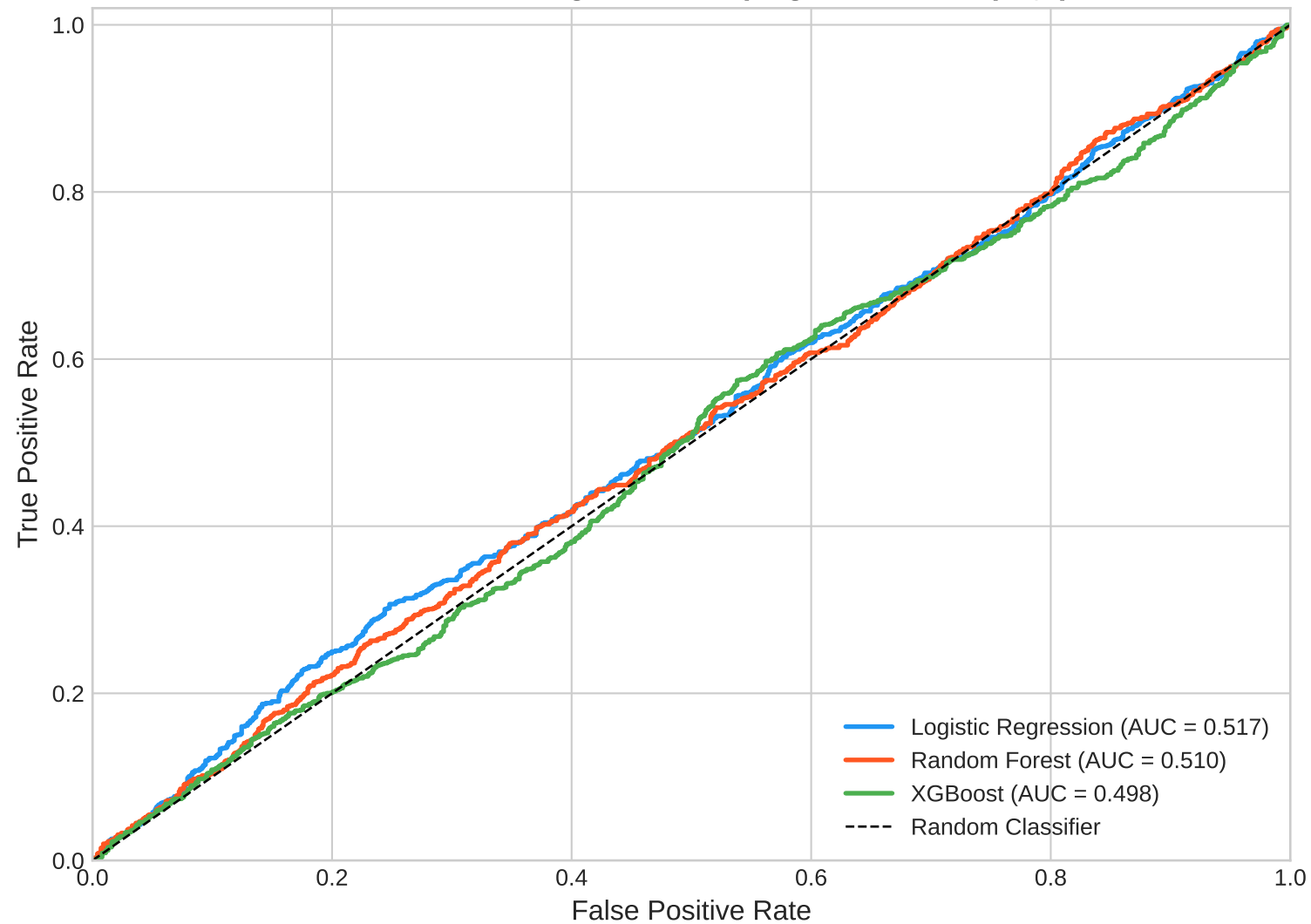
ROC Curves — High-ROI Campaign Prediction (RQ1)
