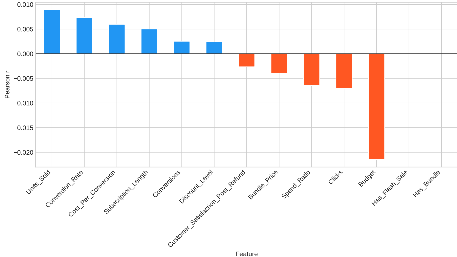
Pearson Correlation with Revenue_Generated (RQ2)
