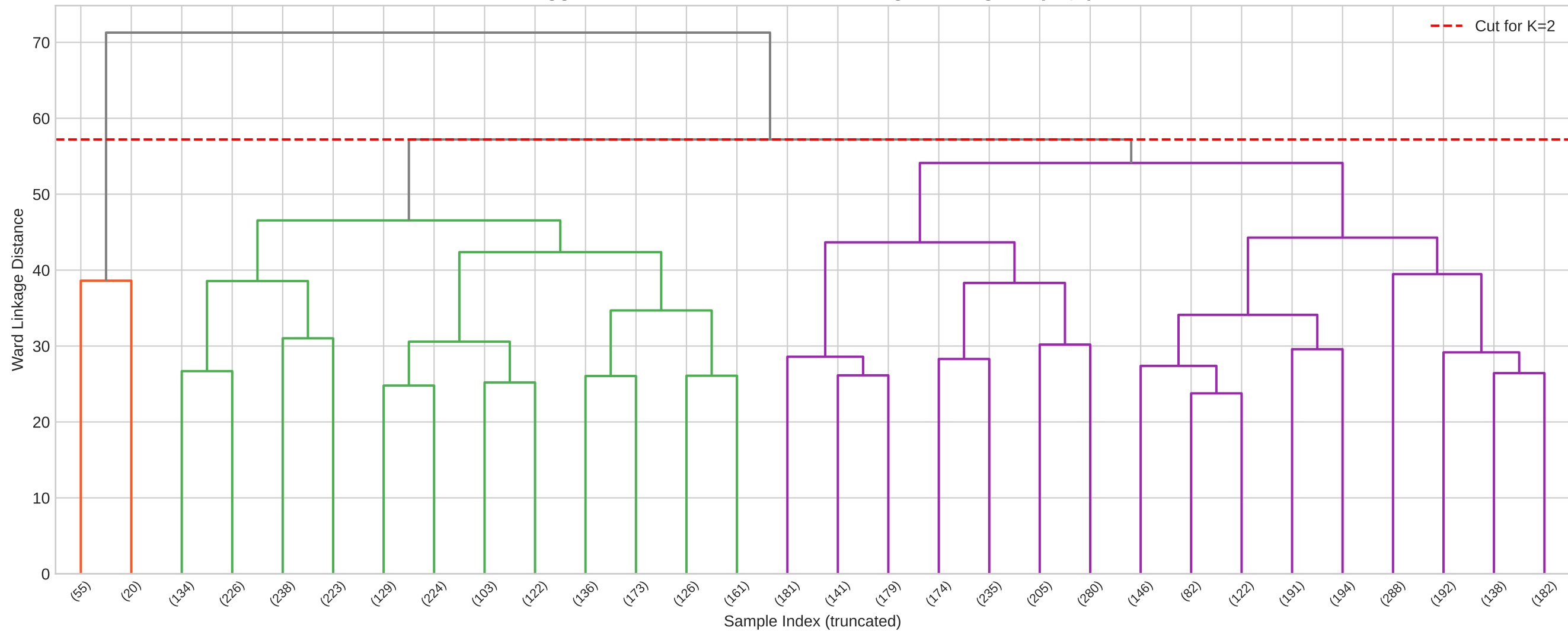
Agglomerative Hierarchical Clustering Dendrogram (RQ3)
