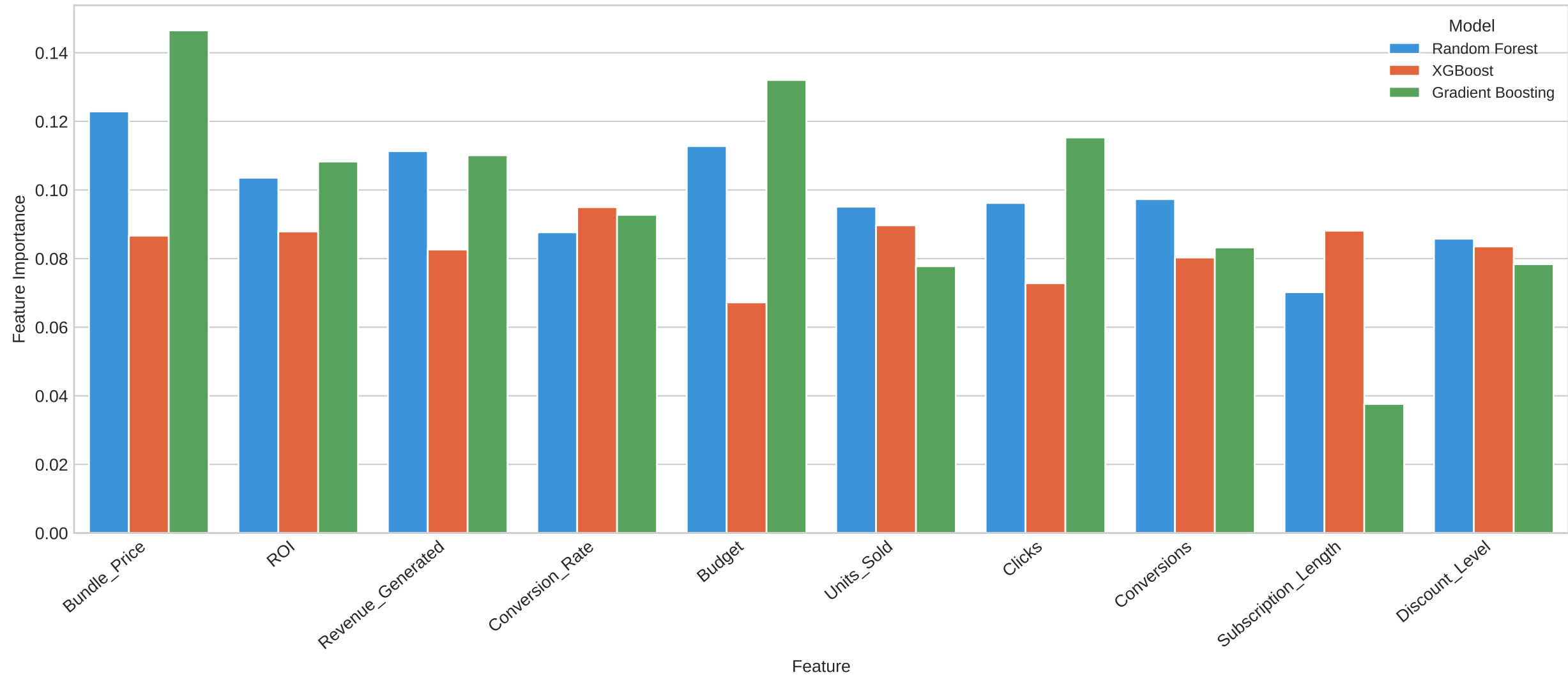
Top-10 Feature Importances by Model (RQ4)
