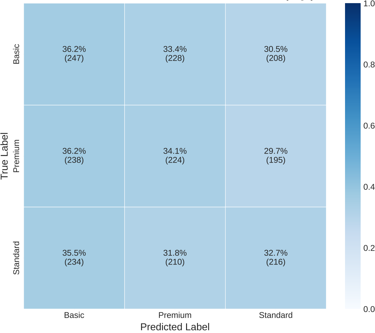
Normalized Confusion Matrix — Random Forest (RQ7)
