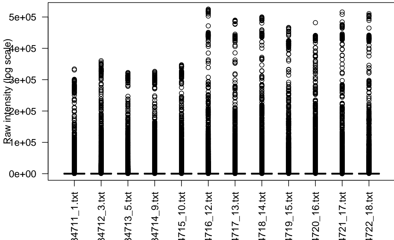
Boxplot: Before Normalization
