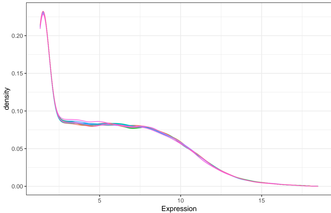
Density plot of normalized log2 expression
