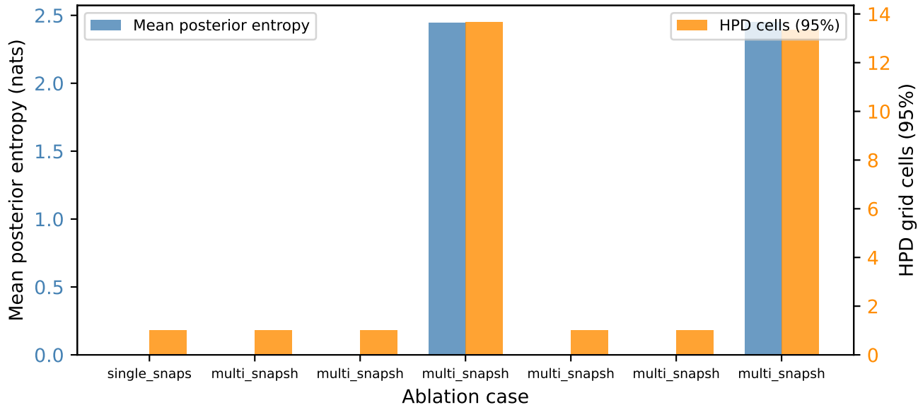
Ablation: Entropy and HPD vs. Case Complexity
