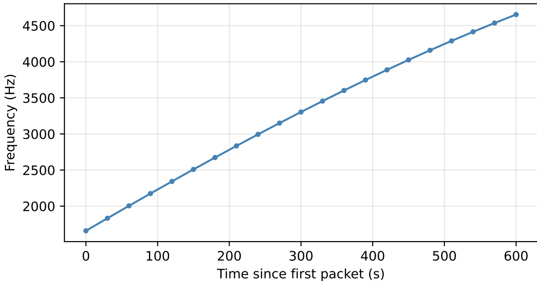
Doppler-Time Fingerprint (from synthetic observations)
