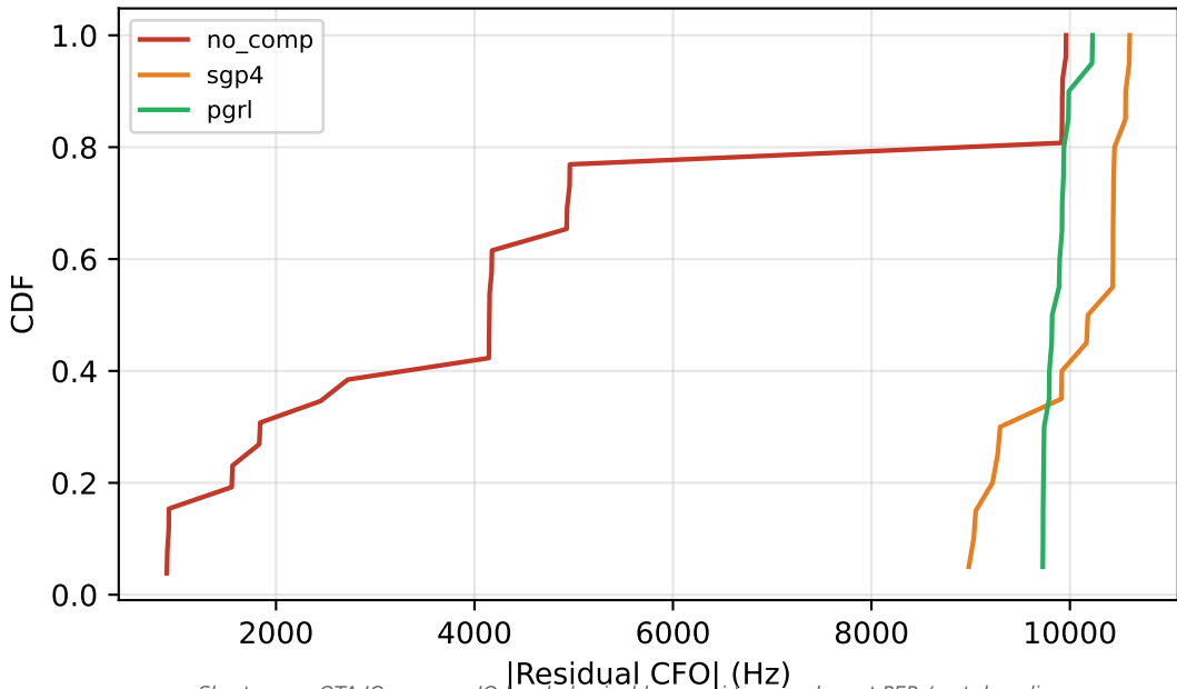
CDF of per-burst residual CFO
