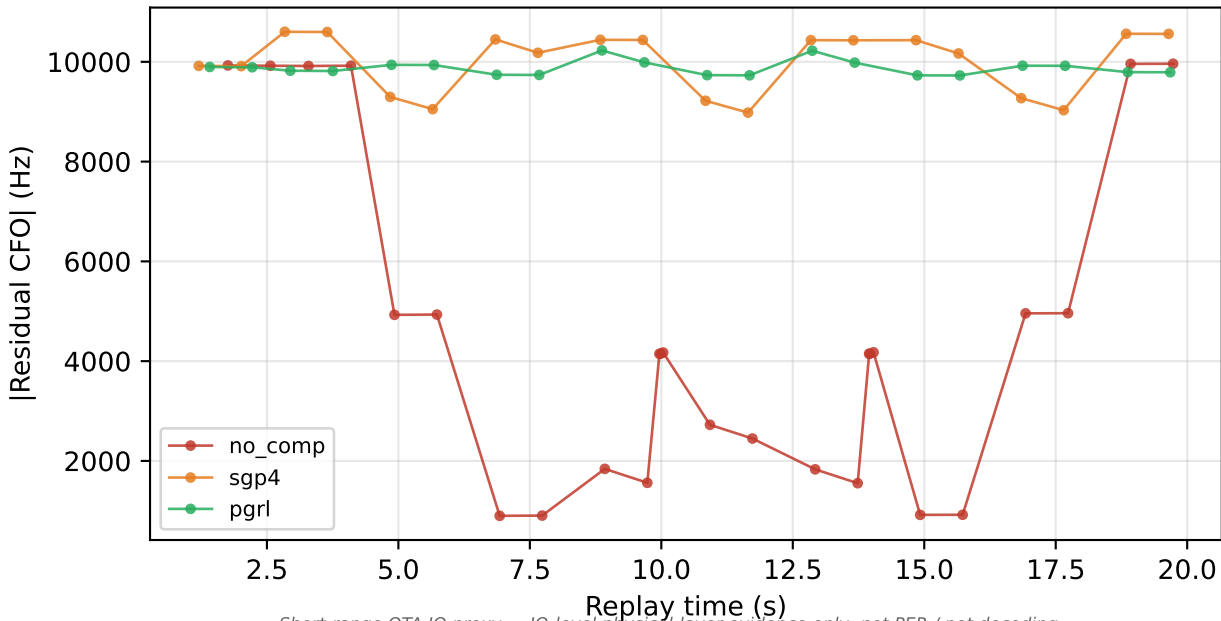
Per-burst residual CFO over replay window
