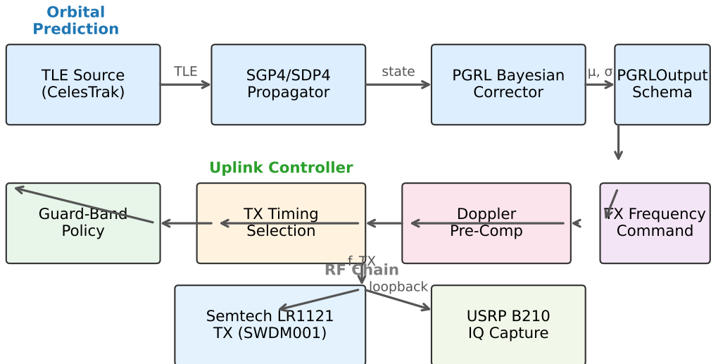
Fig. 1. PGRL-Assisted LR-FHSS Uplink Control: System Architecture
