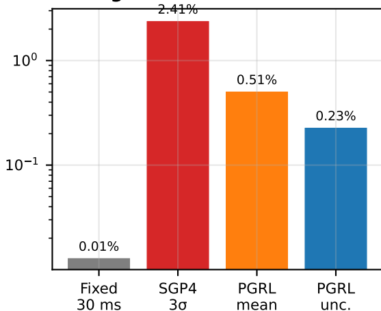
Fig. 3a. Guard Overhead
