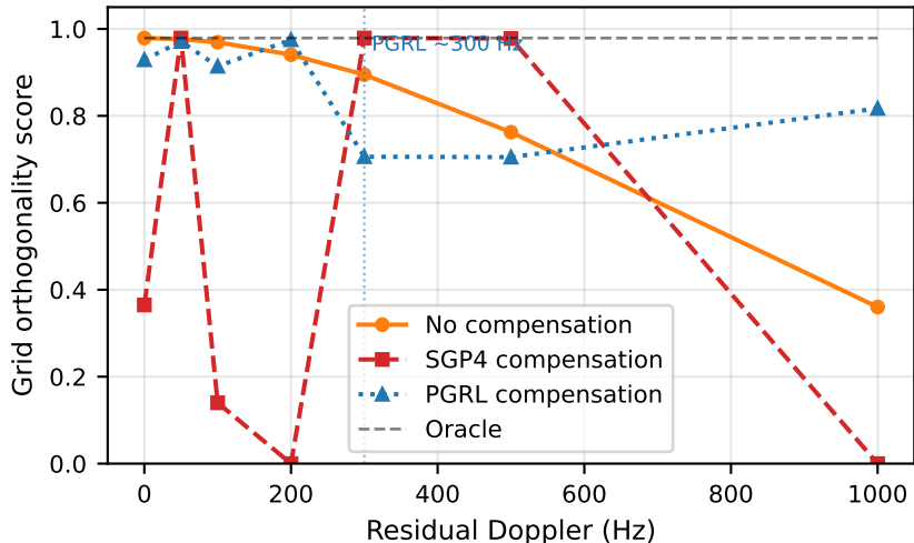
Fig. 4. LR-FHSS Grid Orthogonality vs. Residual Doppler
