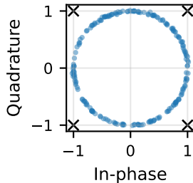
Fig. 5b. QPSK, PGRL, SNR=40 dB (300 Hz residual CFO)
