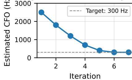
Fig. 5c. CFO Estimation Convergence (Synthetic IQ, SDR dry-run)
