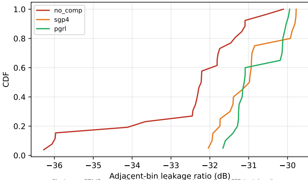
CDF of per-burst adjacent-bin leakage
