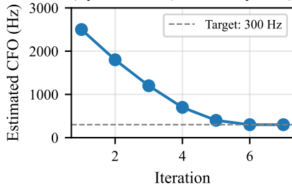
Fig. 5c. CFO Estimation Convergence (Synthetic IQ, SDR dry-run)
