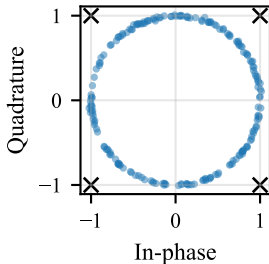
Fig. 5b. QPSK, PGRL, SNR=40 dB (300 Hz residual CFO)
