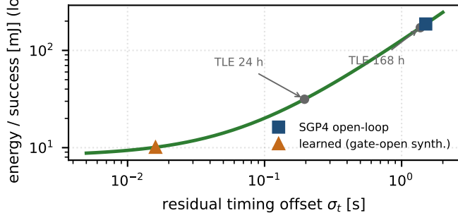
(b) energy vs. timing offset
