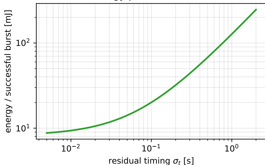
(c) Energy per successful burst
