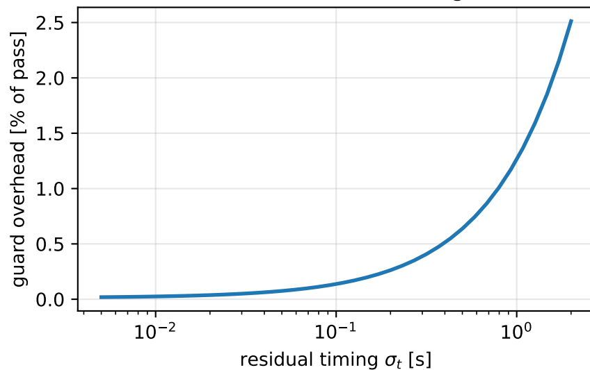
(b) Guard overhead vs timing offset
