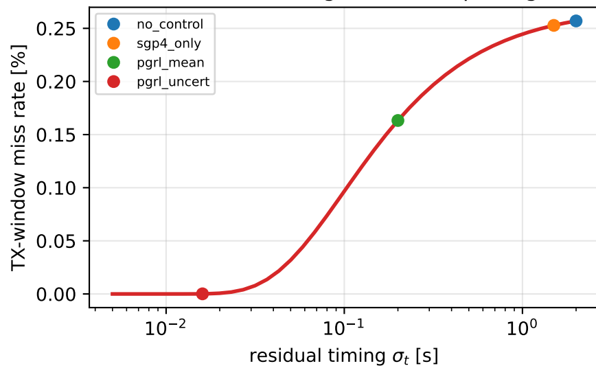
(a) Miss rate vs timing offset (adaptive guard)
