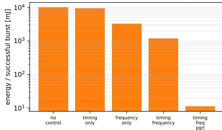
(d) Energy per successful burst (log, capped 10^4 )
