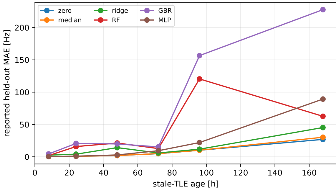
Stronger baseline comparison (reported test metrics)
